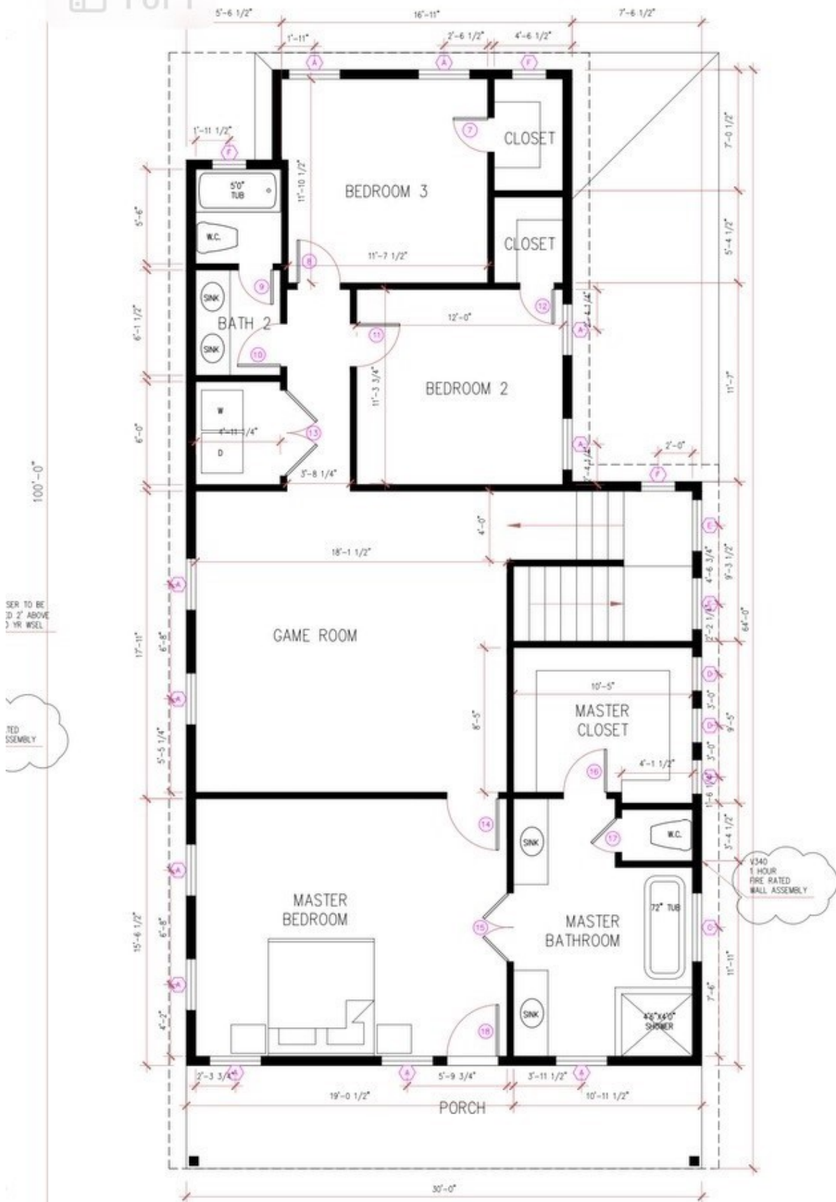
2 SECOND FLOOR PLAN A2 SCALE: 1/4" = 1'-0"
