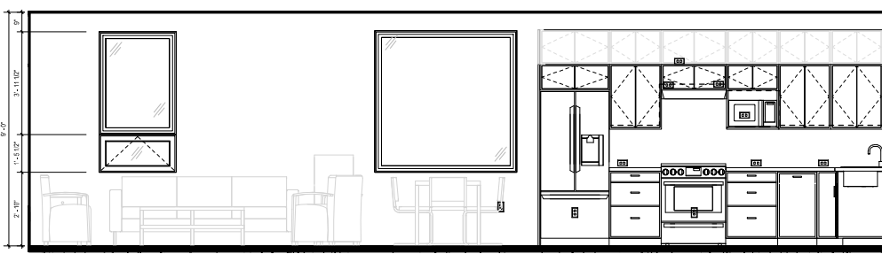
UNIT C - WINDOW ELEVATION "F" SCAL. 1/2" = 1'-0" 6
