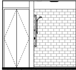
M. BATH ELEVATION - 2 | SCAL. 1/2" = 1'-0" | 8
