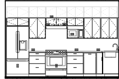
KITCHEN ELEVATION - 1 | SCAL. 1/2" = 1'-0" | 5
