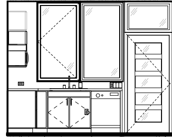
KITCHEN ELEVATION - 2 | SCAL. 1/2" = 1'-0" | 6
