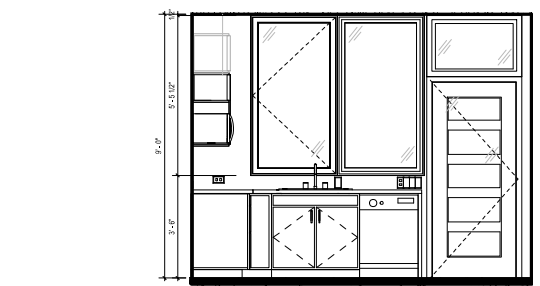
UNIT C - WINDOW ELEVATION "B" SCAL. 1/2" = 1'-0" 2
