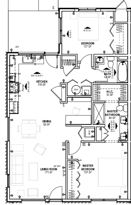
UNIT C - FLOOR PLAN | SCAL. 1/4" = 1'-0" | 1
