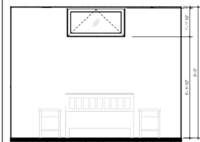
UNIT C - WINDOW ELEVATION "A" (OPT. 1) SCAL. 1/2" = 1'-0" 1
