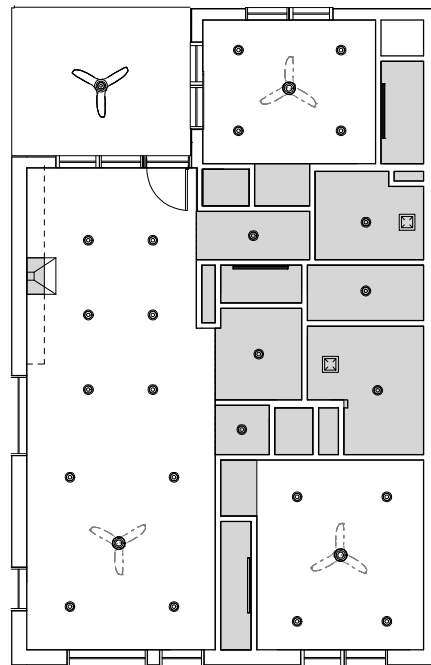
REFLECTED CEILING PLAN | SCAL. 1/4" = 1'-0" | 2
