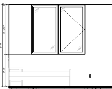
UNIT C - WINDOW ELEVATION "C" SCAL. 1/2" = 1'-0" 3
