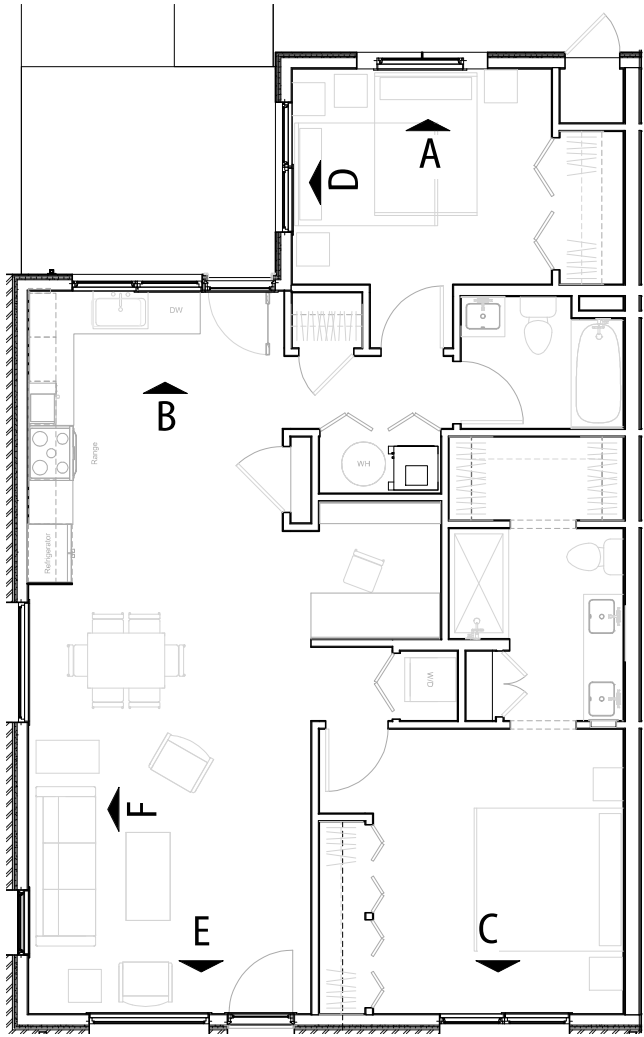
UNIT C - ELEVATION REFERENCE PLAN SCAL. 3/8" = 1'-0" 7
