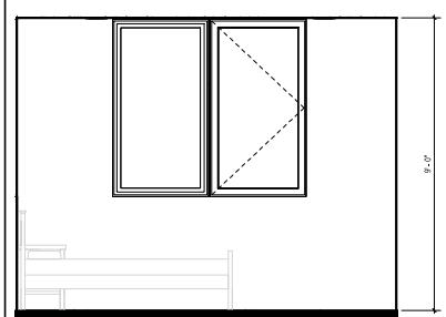
UNIT C - WINDOW ELEVATION "A" (OPT. 2) SCAL. 1/2" = 1'-0" 8
