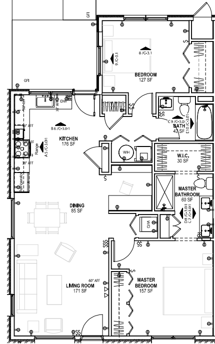
UNIT C - FLOOR PLAN (OPTION 2) | SCAL. 1/4" = 1'-0" | 4
