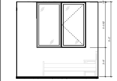
UNIT C - WINDOW ELEVATION "D" (OPT. 1) SCAL. 1/2" = 1'-0" 4
