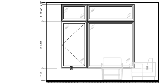
UNIT C - WINDOW ELEVATION "E" SCAL. 1/2" = 1'-0" 5
