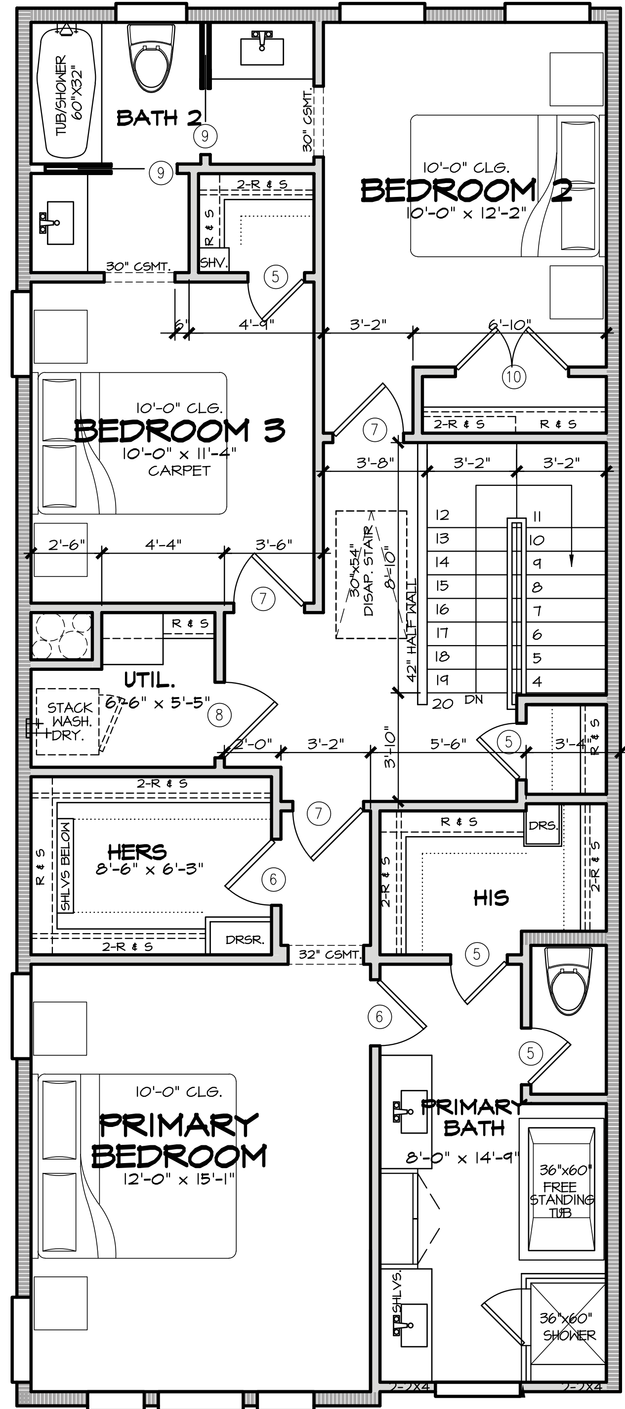
SECOND FLOOR
