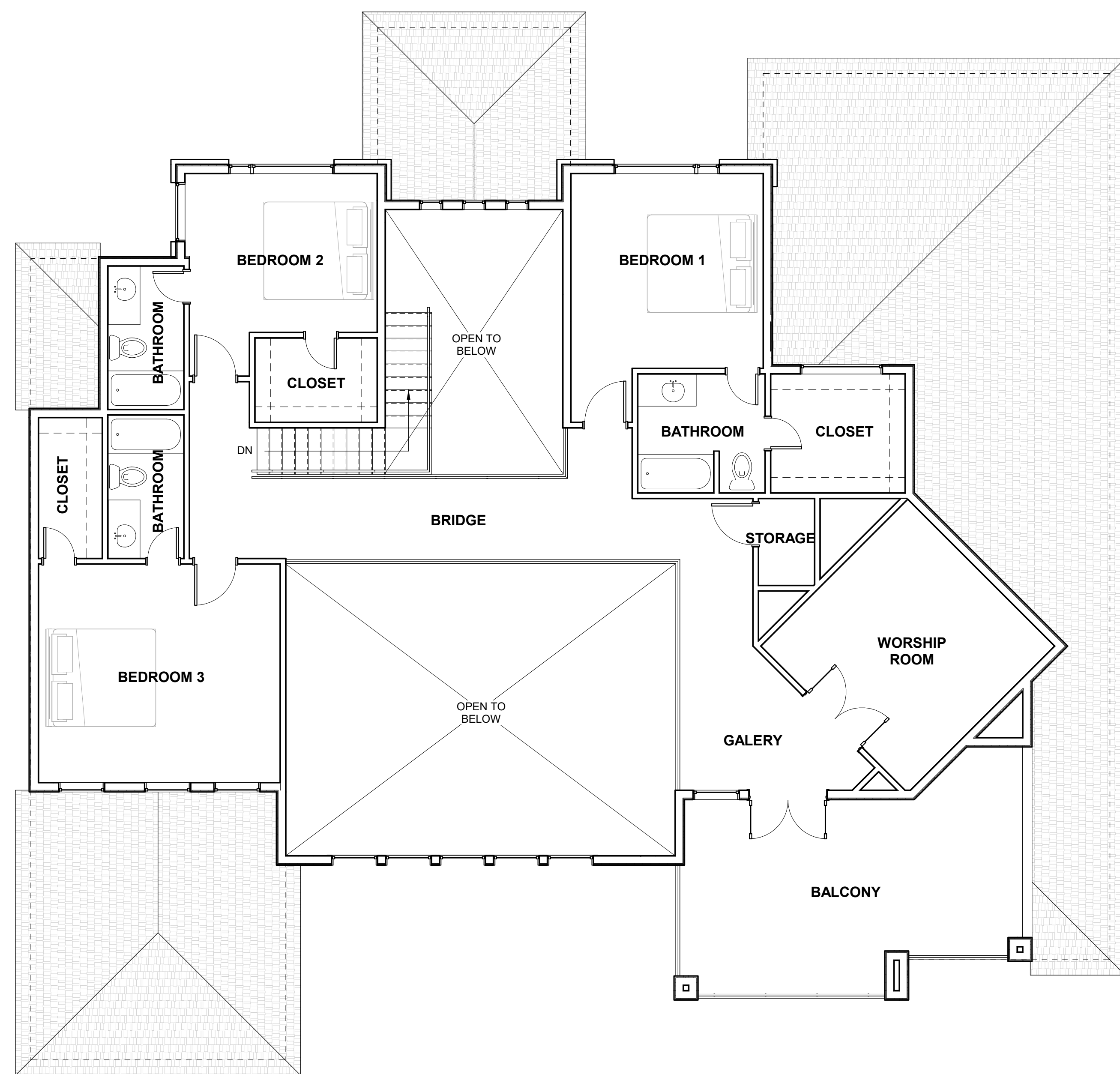
2 SECOND FLOOR PLAN 3/16" = 1'-0"
