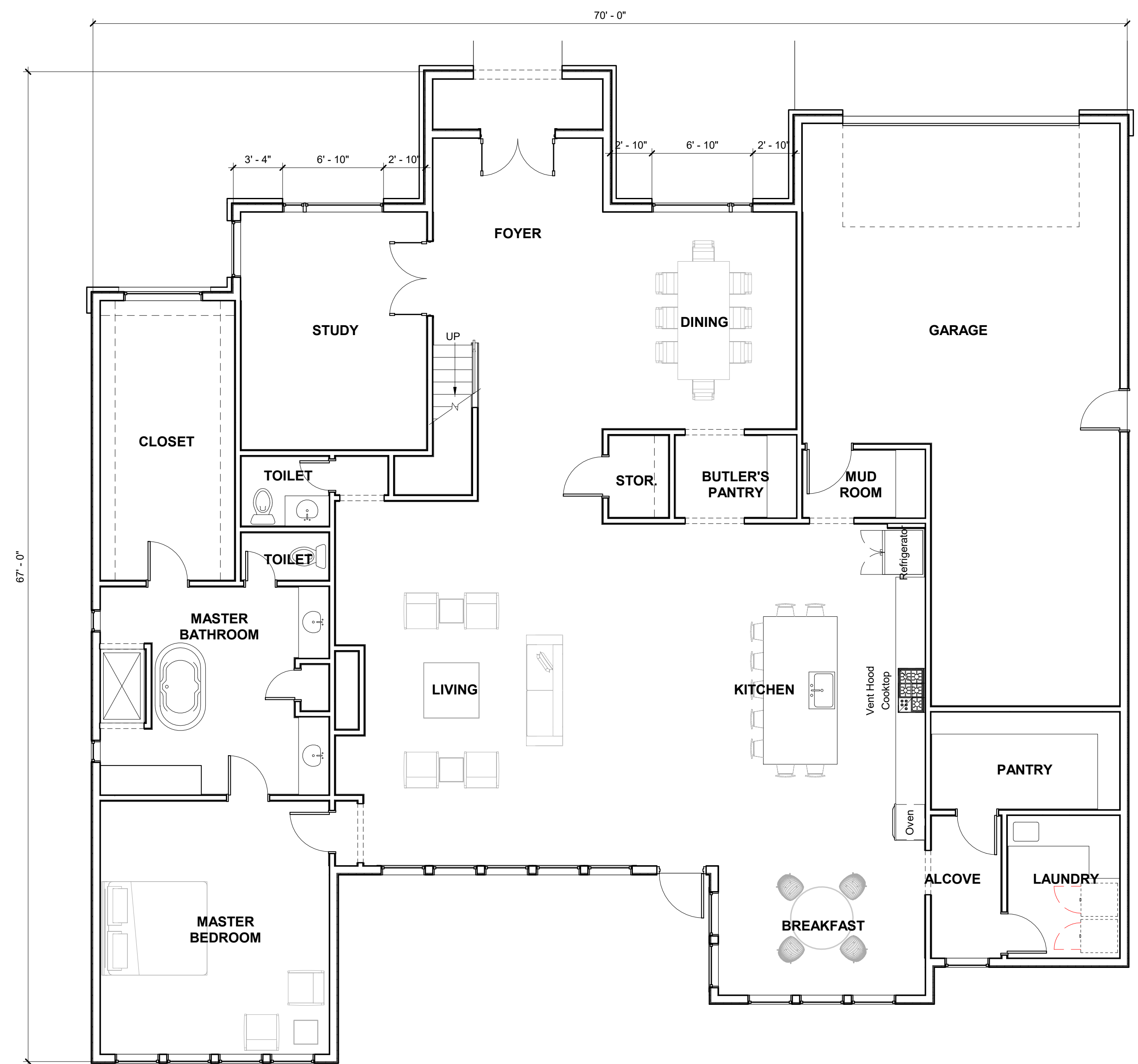
1 FIRST FLOOR PLAN 3/16" = 1'-0"
