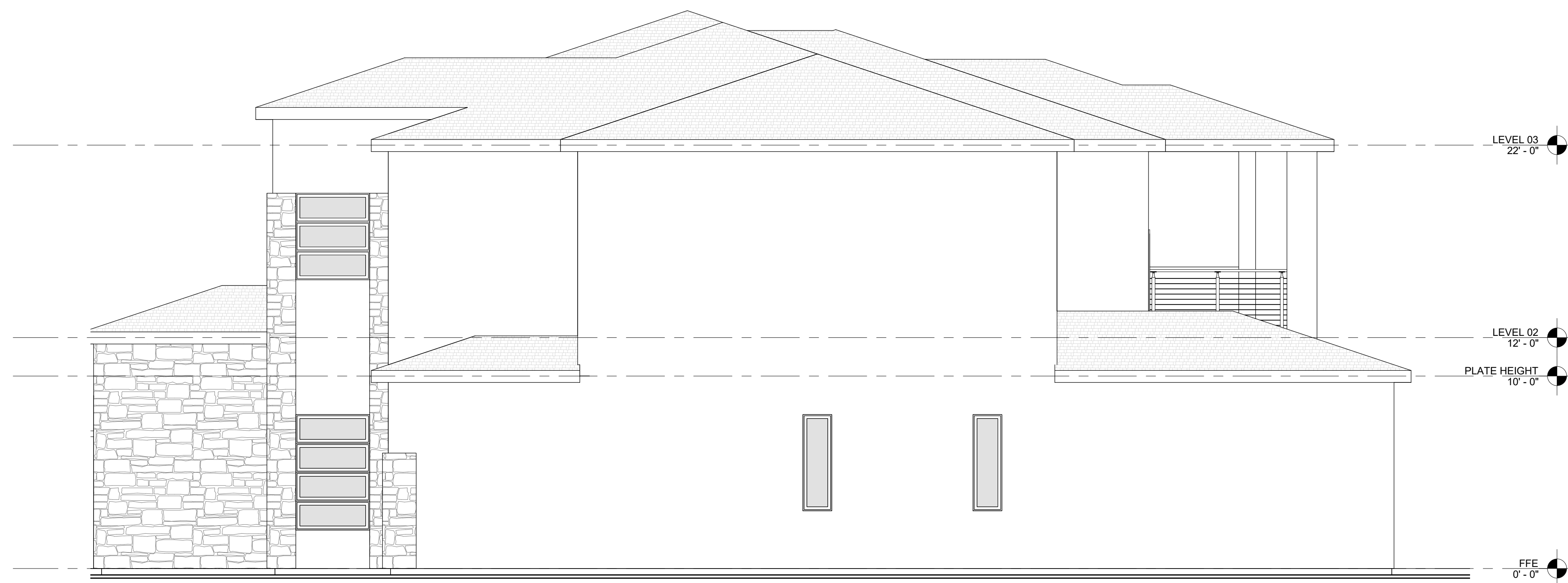
2 WEST ELEVATION 1/4" = 1'-0"
