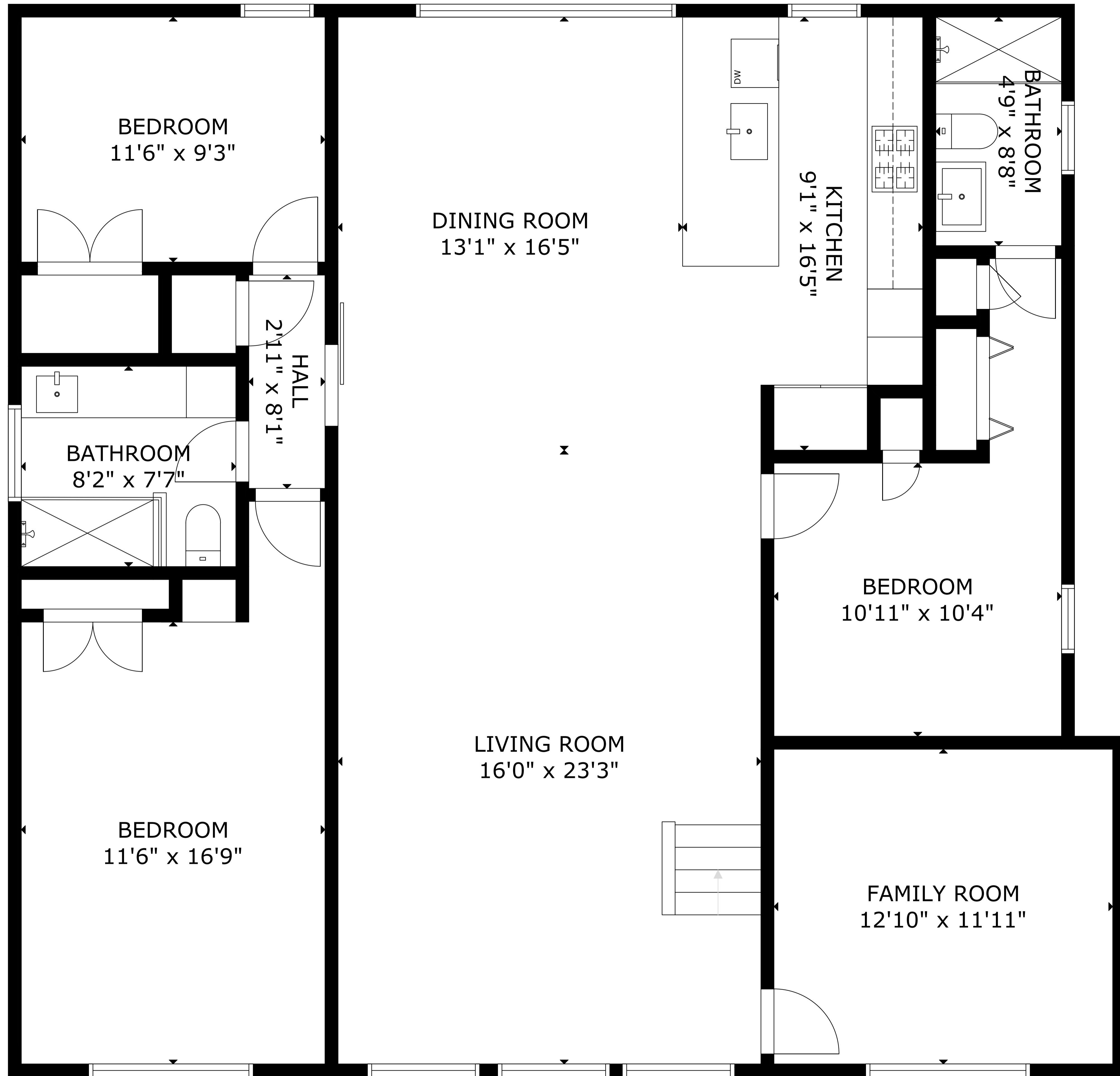
FLOOR 1
