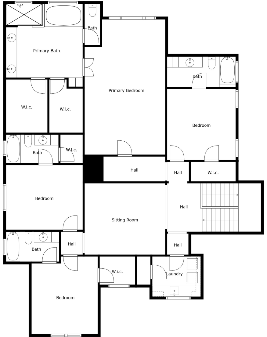
Floor 2
