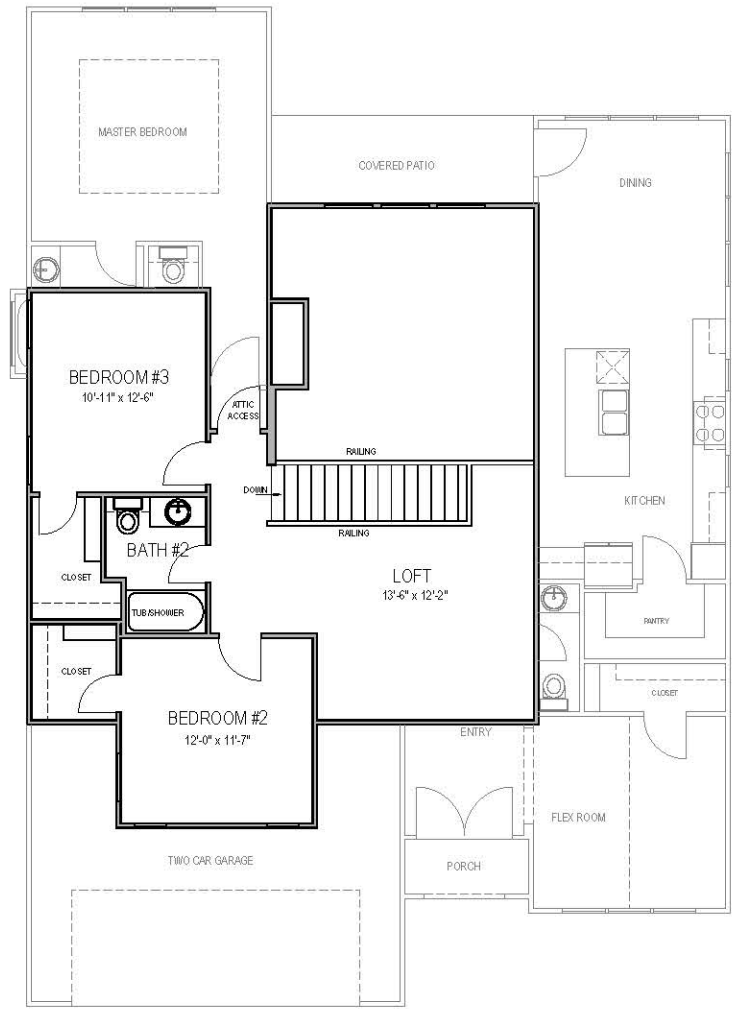
SECOND FLOOR
