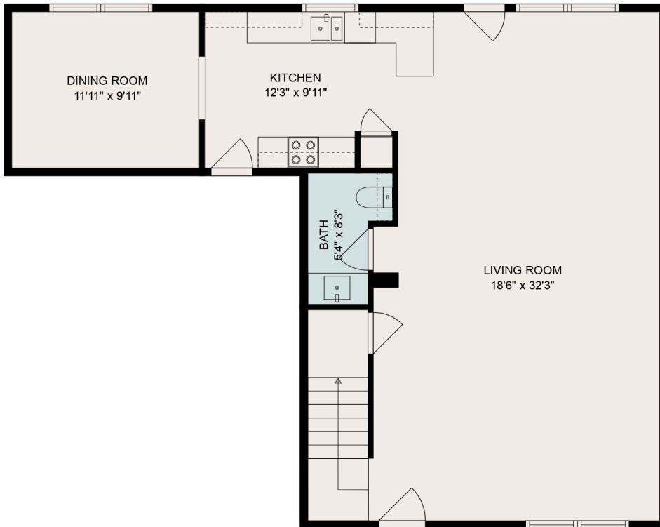
FLOOR 1
