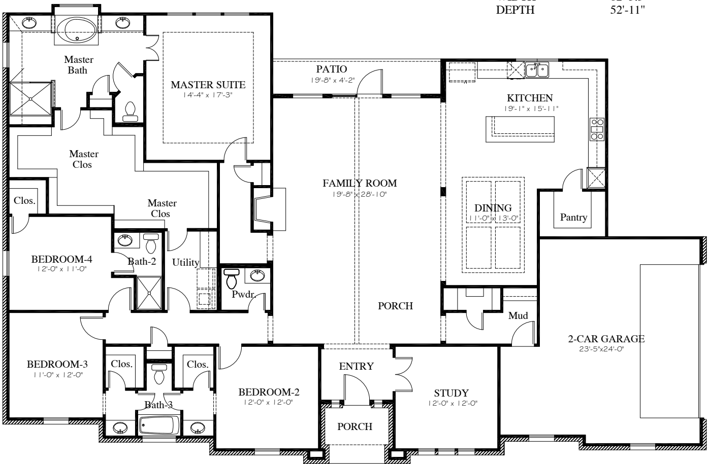
FLOOR PLAN
