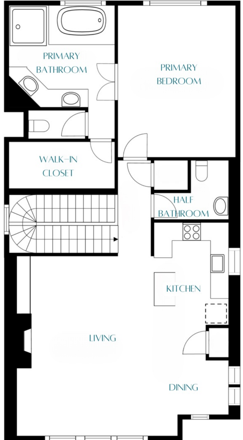
SECOND FLOOR
