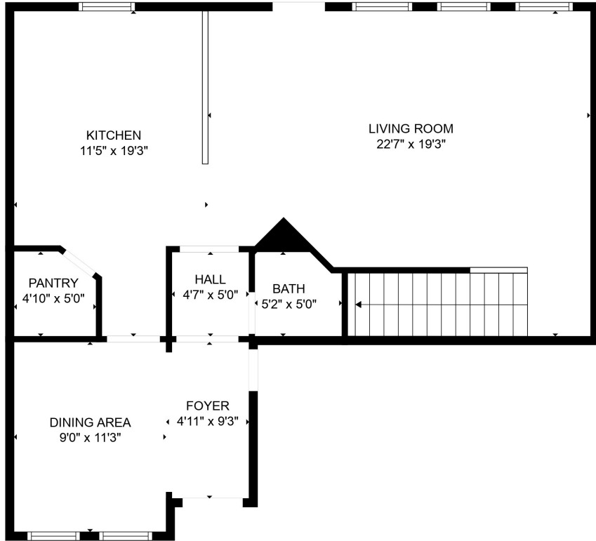
FLOOR 1
