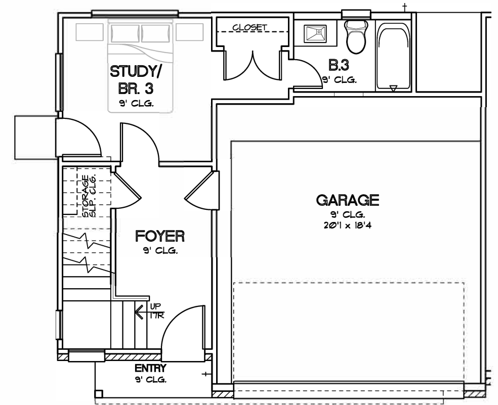
FIRST FLOOR PLAN PLAN 1781
