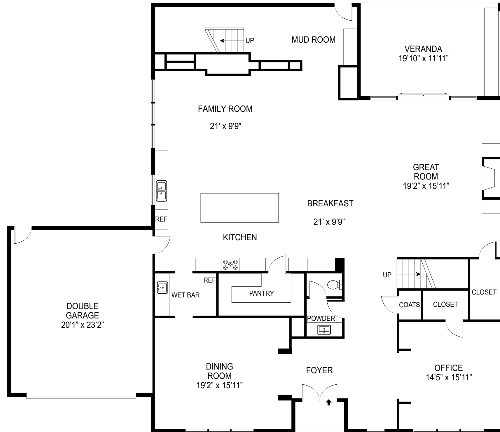
FIRST FLOOR
