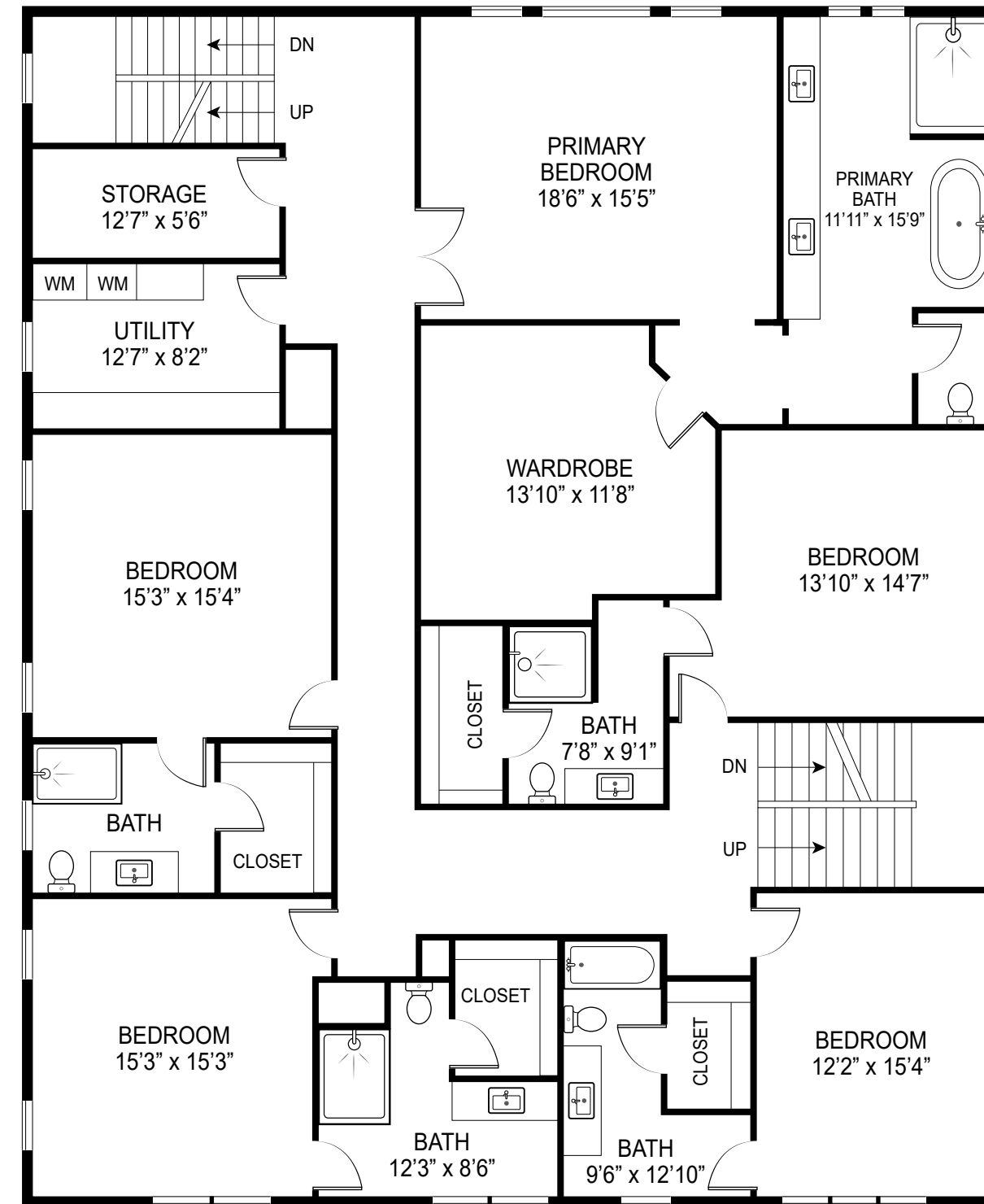
SECOND FLOOR
