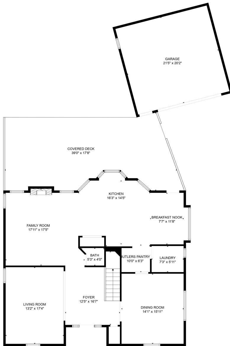
FLOOR 1
