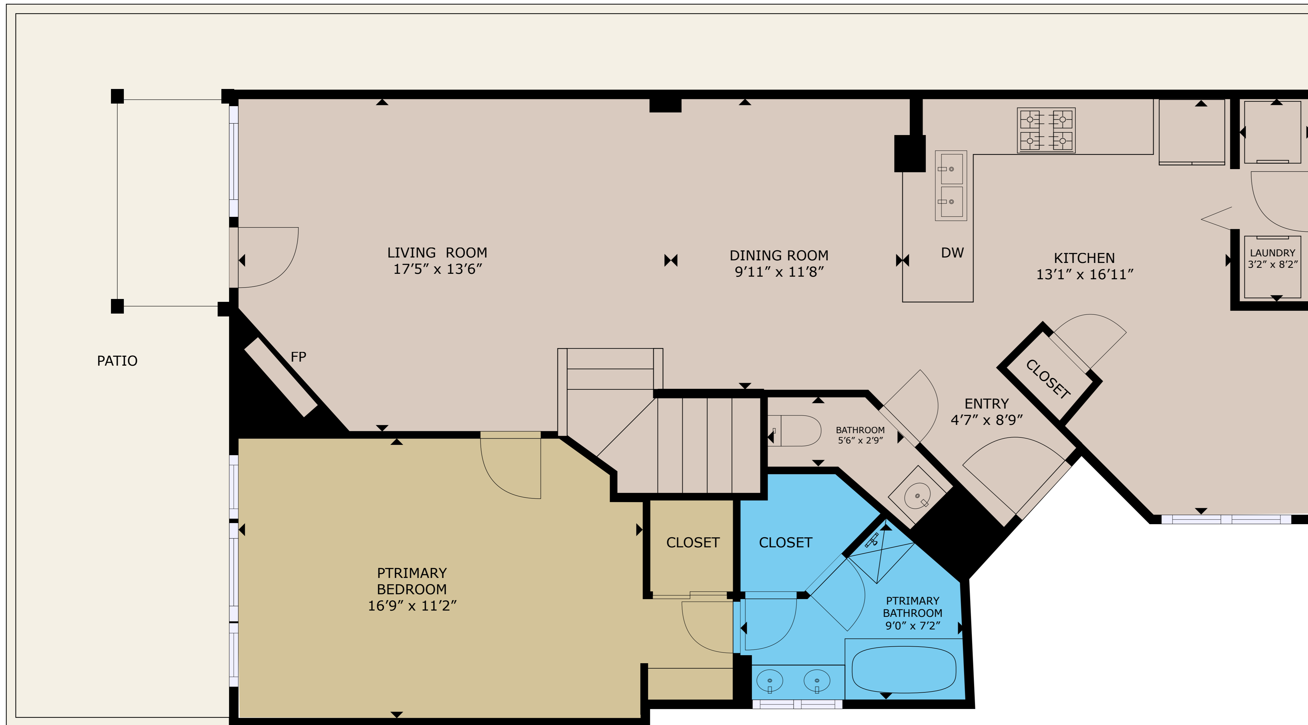
FLOOR 1
