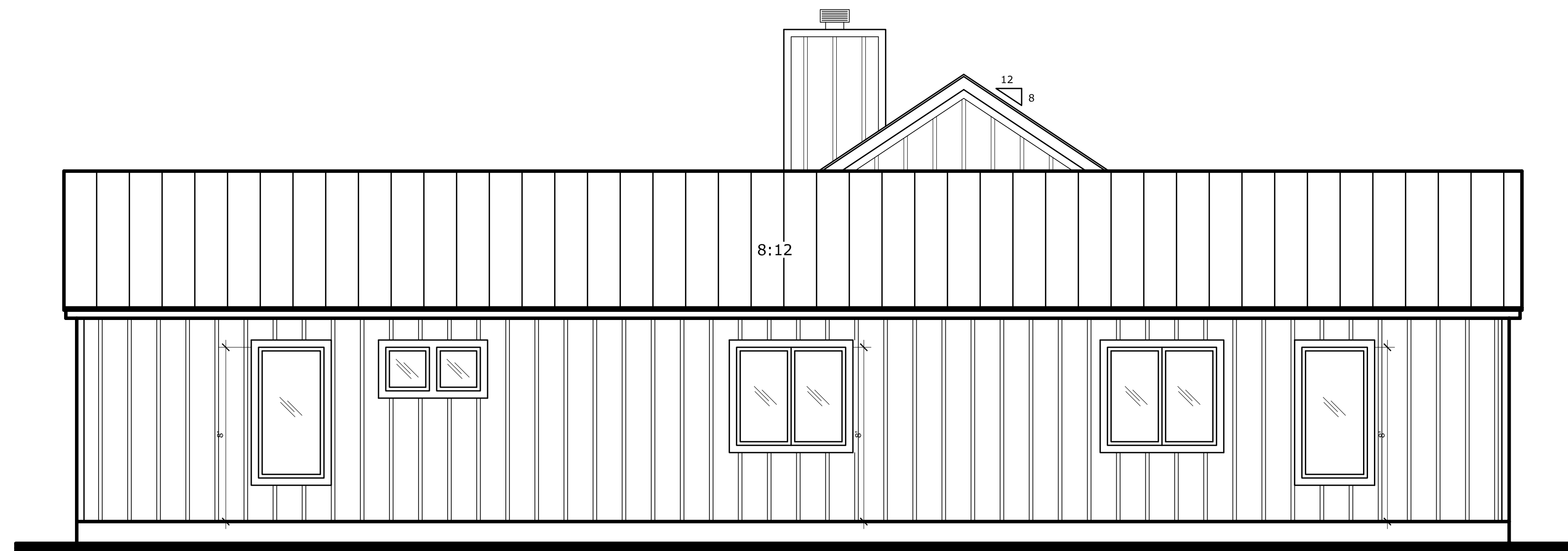
LEFT ELEVATION
