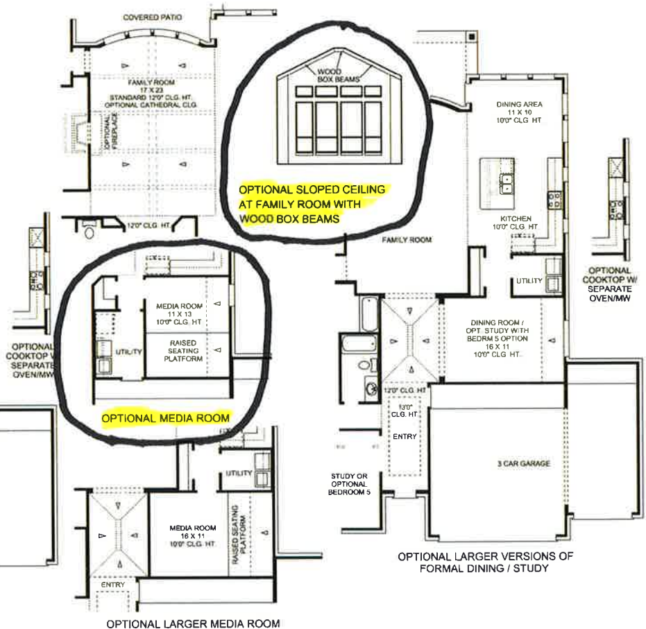
floor plan options
