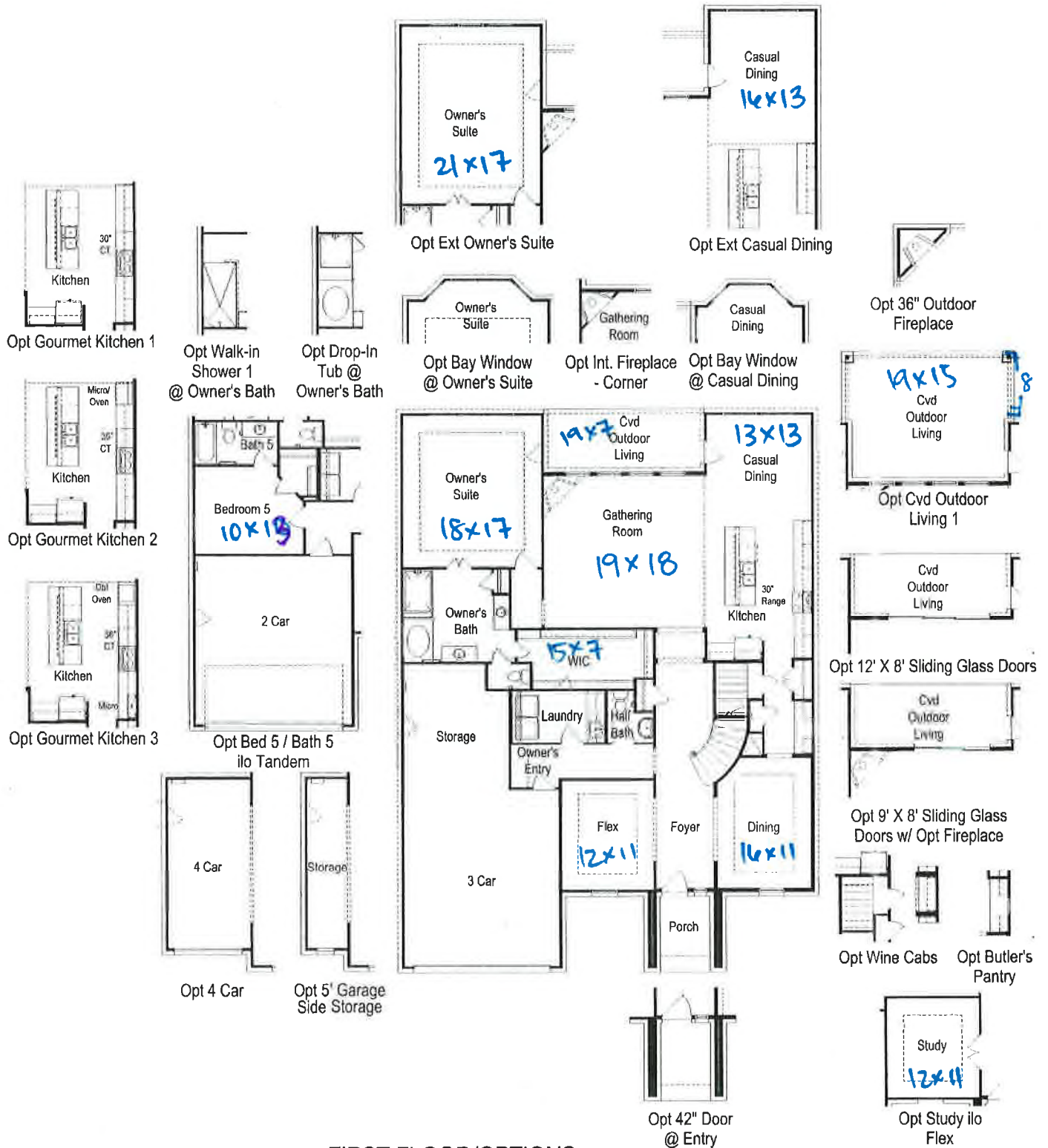
FIRST FLOOR/OPTIONS
