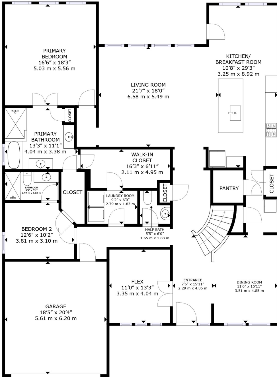
FLOOR 1
