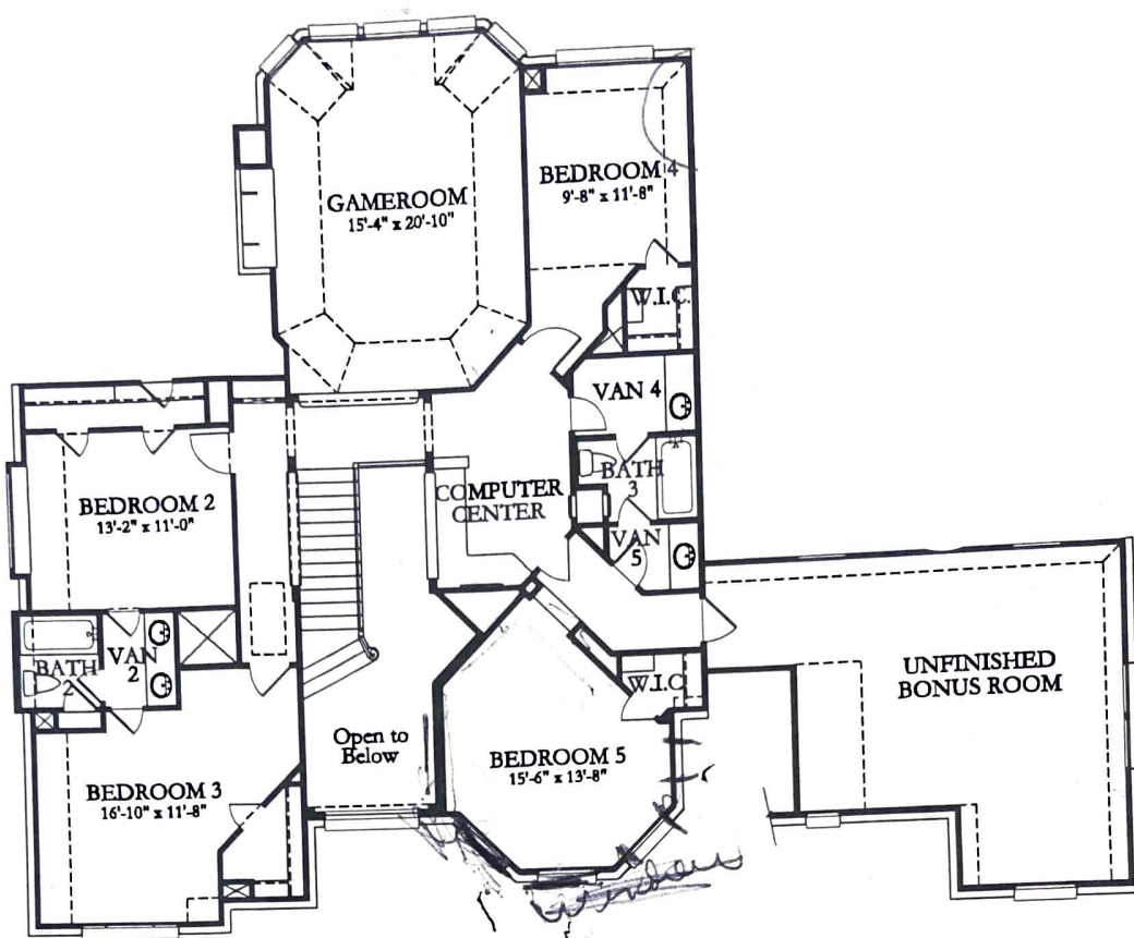
SECOND FLOOR
