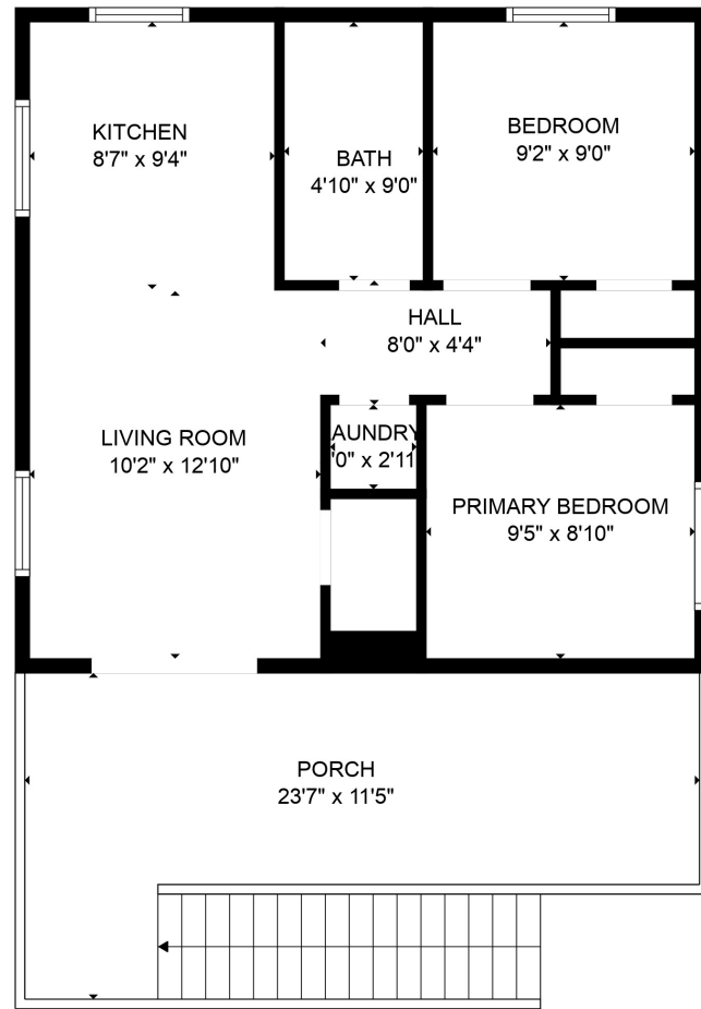
FLOOR 2
