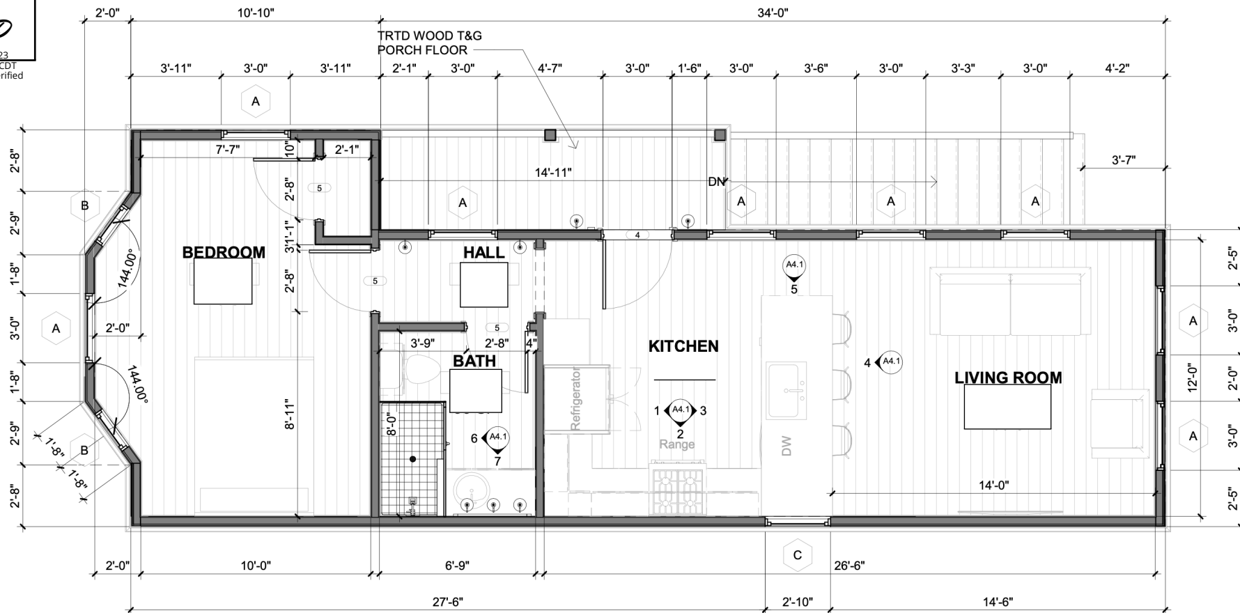
② Garage Apartment 1/4" = 1'-0"
