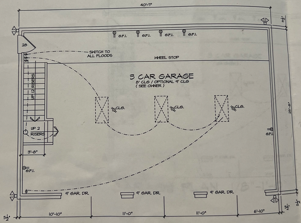
GARAGE PLAN 1/8"-1'-0"
