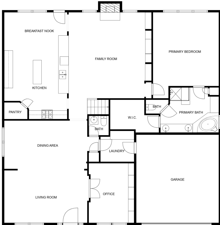
FLOOR 1
