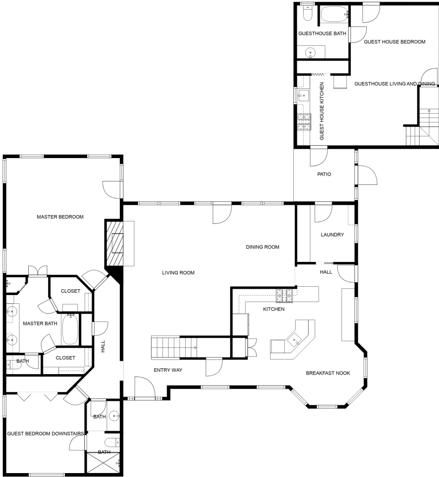
FLOOR 1
