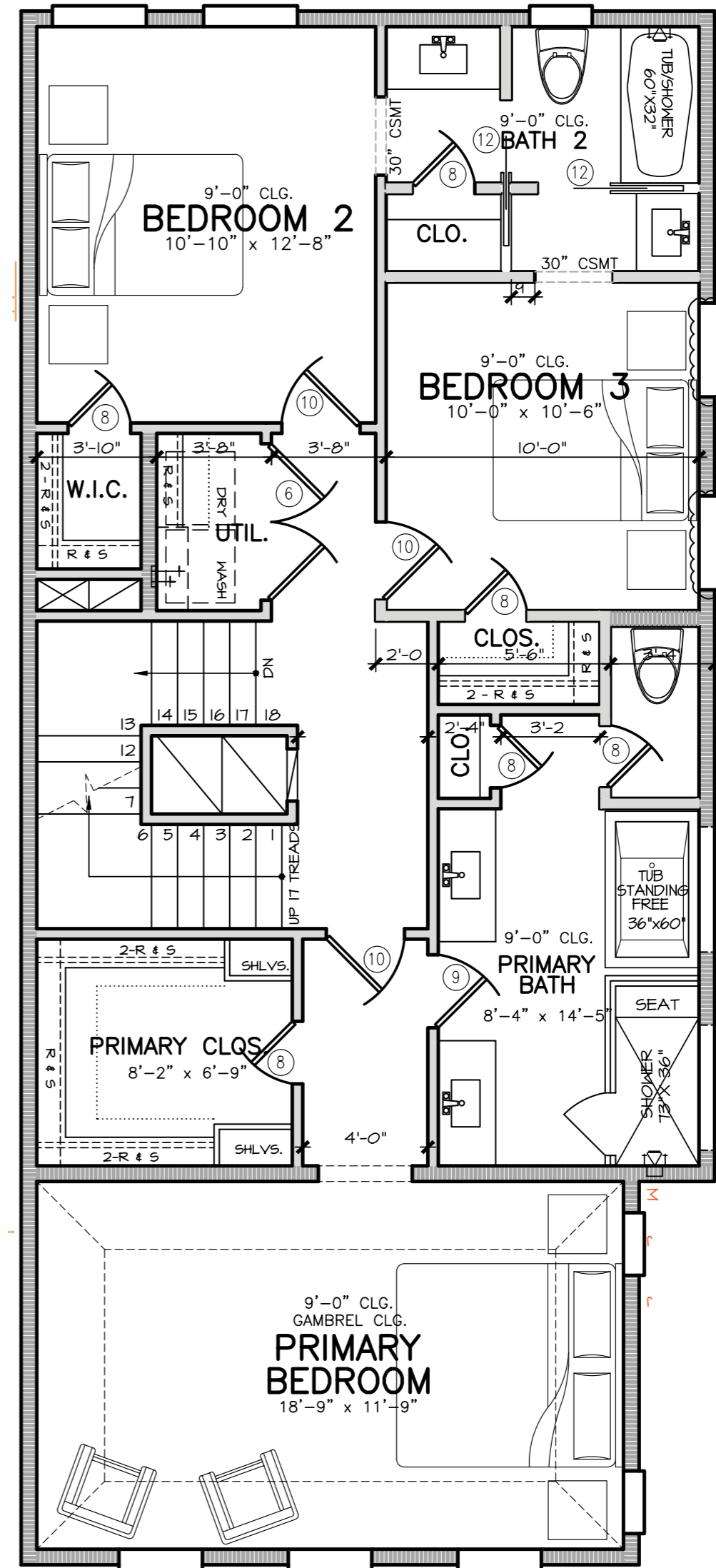
SECOND FLOOR
