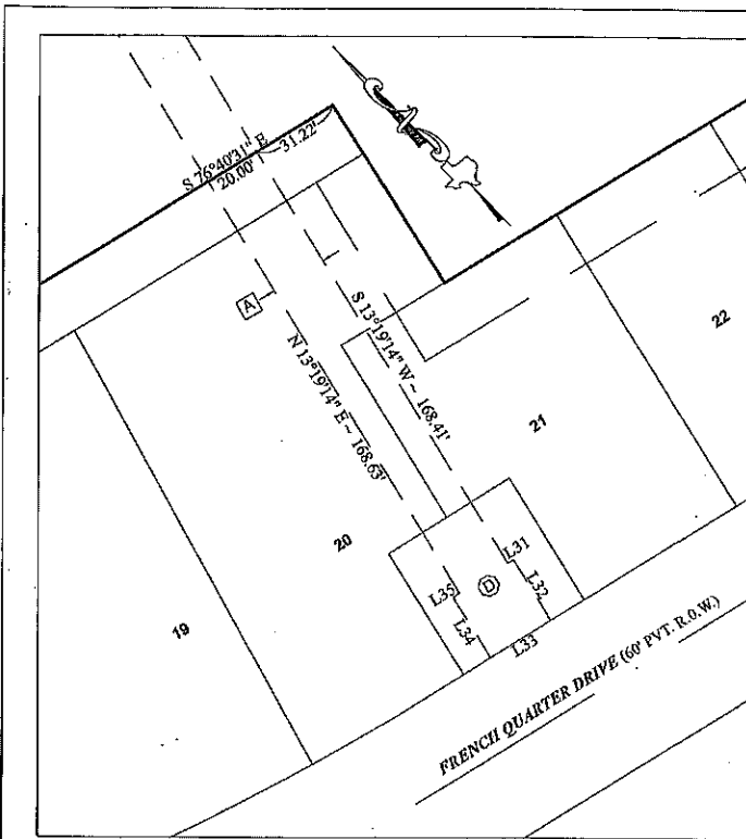
DETAIL "A" SCALE 1" = 40'
