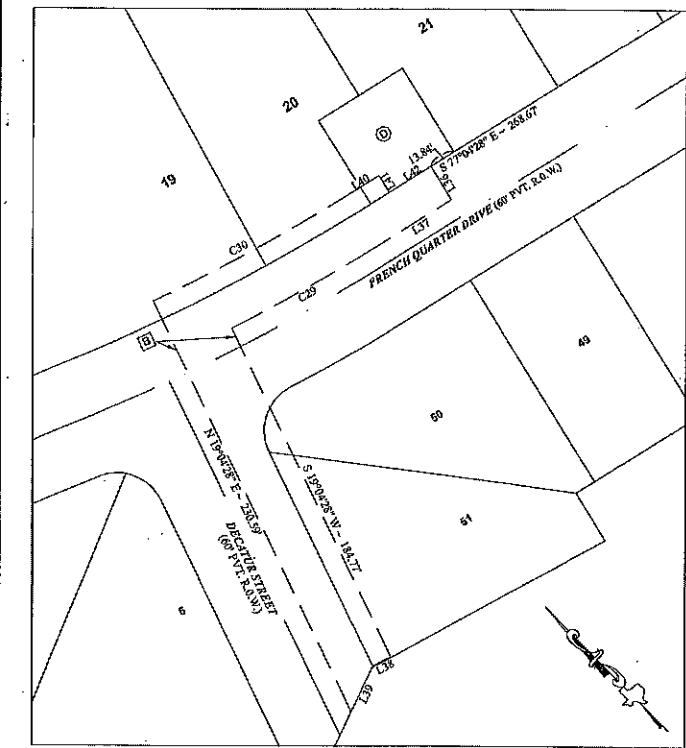
DETAIL "B" SCALE 1" = 40'
