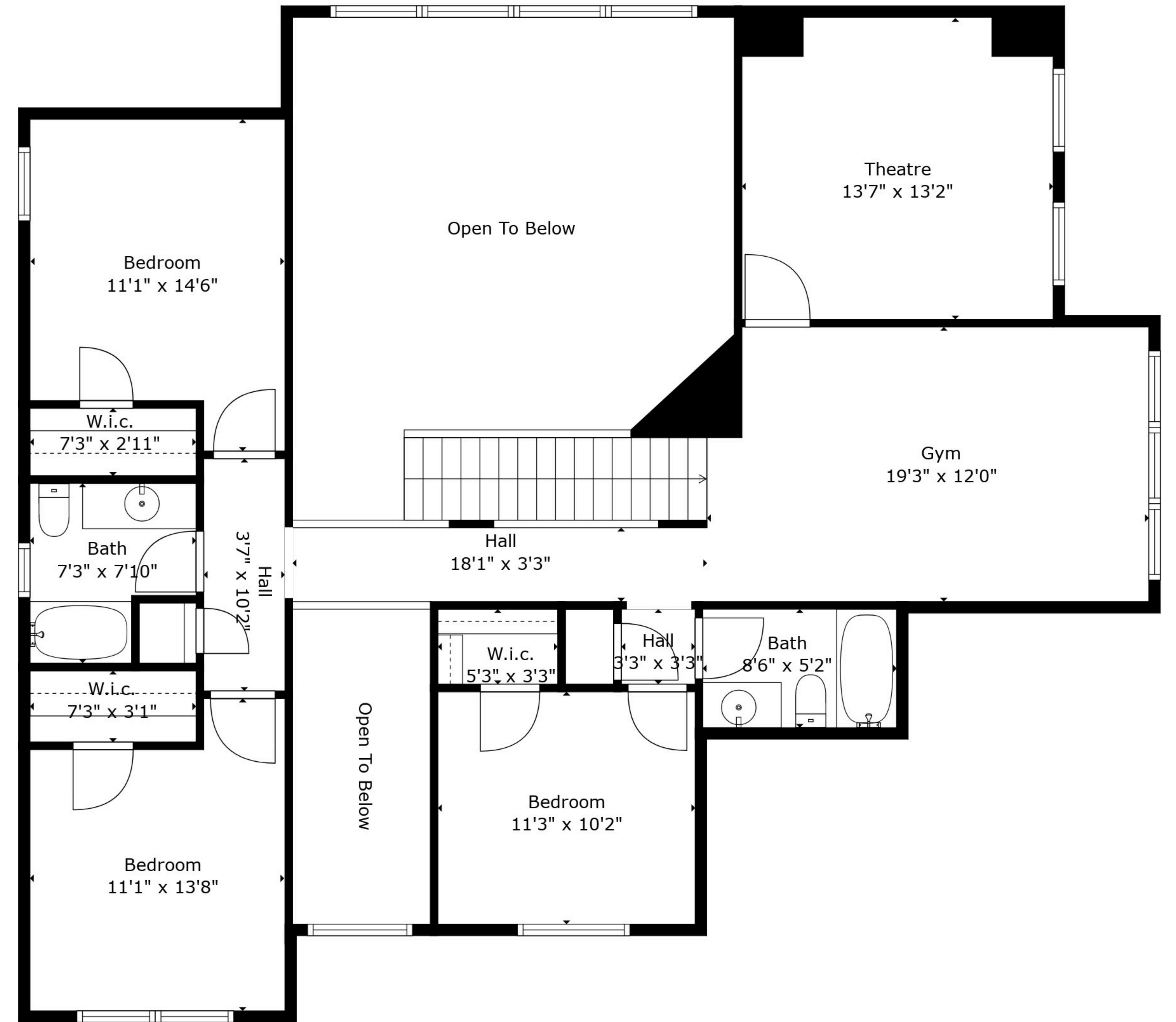
Floor 2
