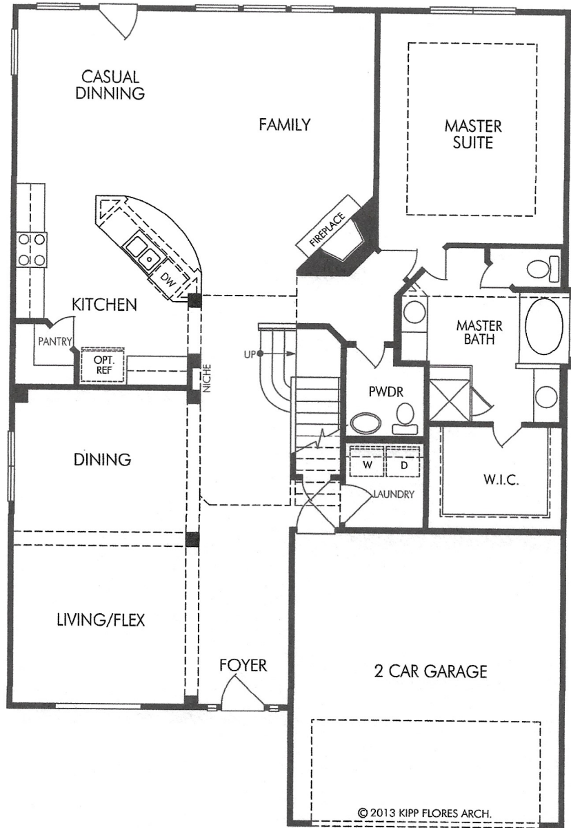
FLOOR PLAN
