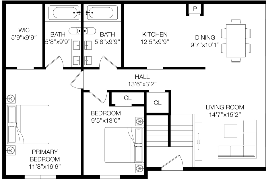
FLOOR 2
