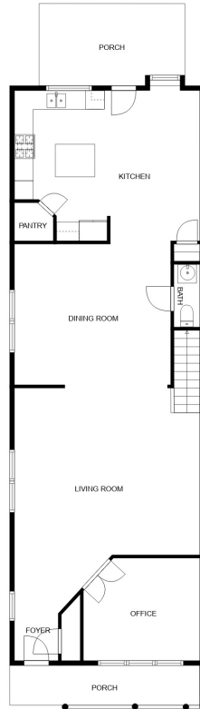
FLOOR 1
