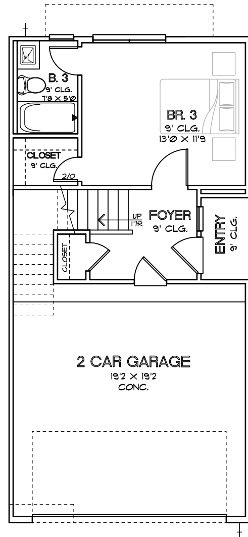
FIRST FLOOR PLAN PLAN 1905 R
