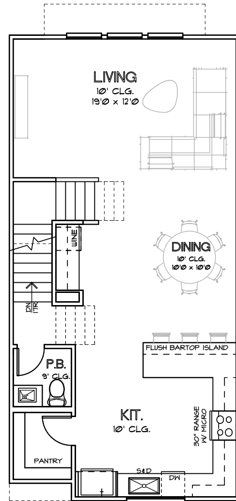
SECOND FLOOR PLAN PLAN 1905 R
