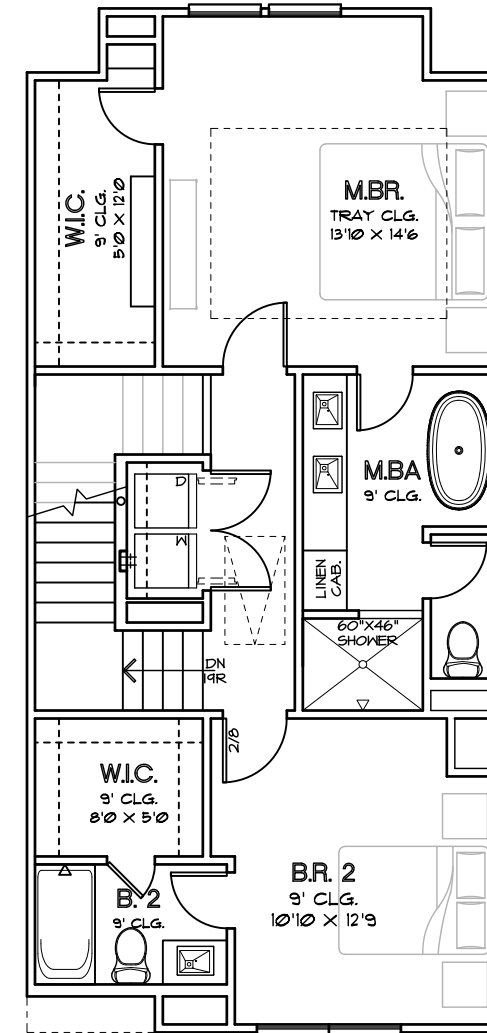
THIRD FLOOR PLAN PLAN 1905 R
