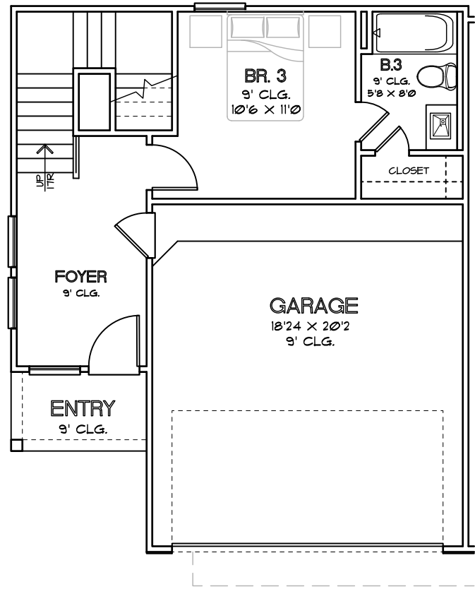
FIRST FLOOR PLAN PLAN 1968
