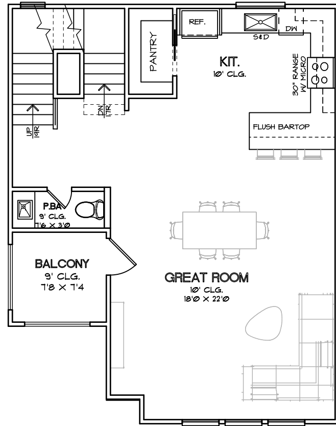
SECOND FLOOR PLAN PLAN 1968
