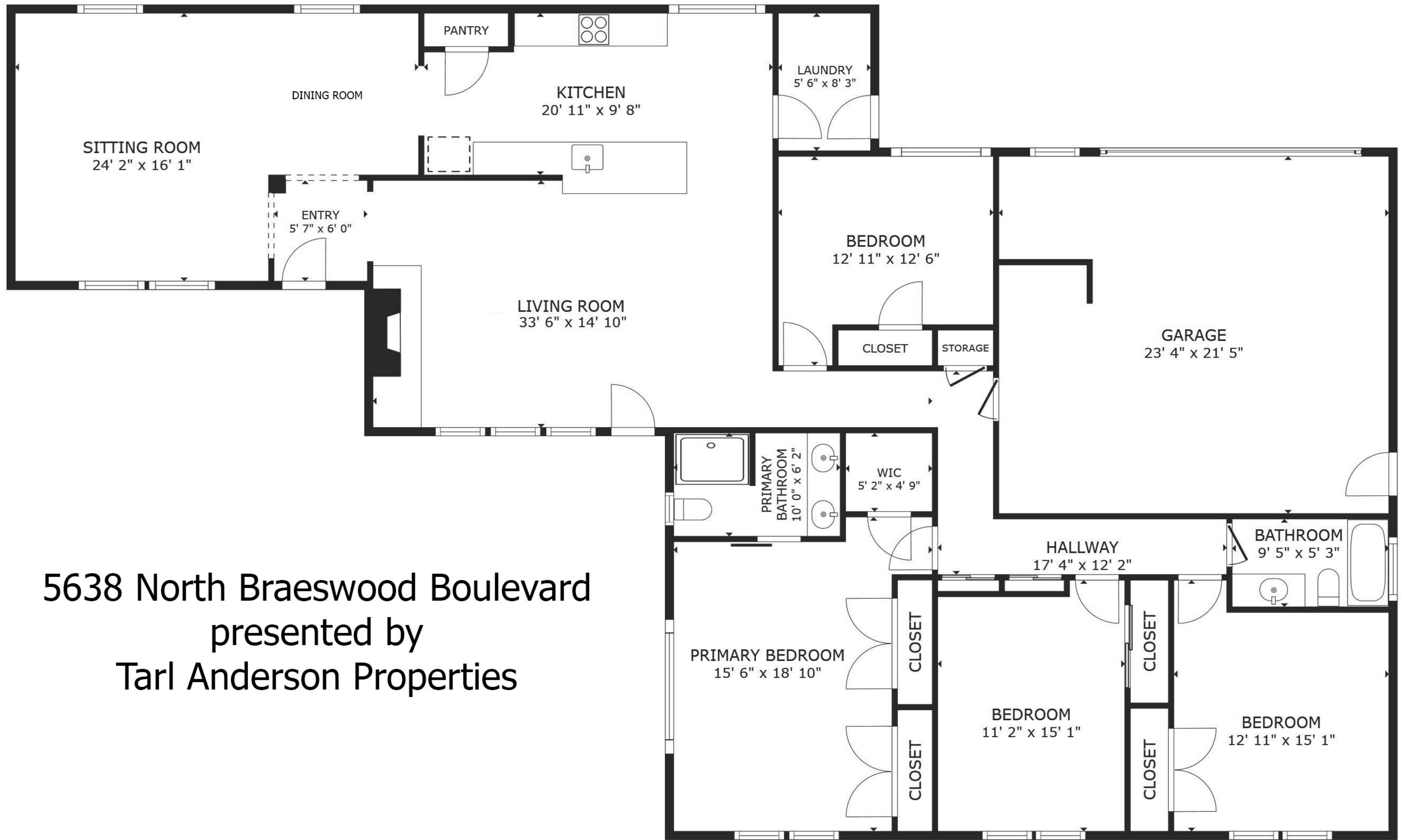
FLOOR PLAN
