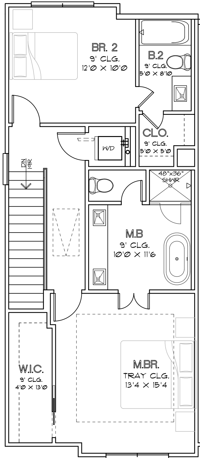
THIRD FLOOR PLAN PLAN 1870 L
