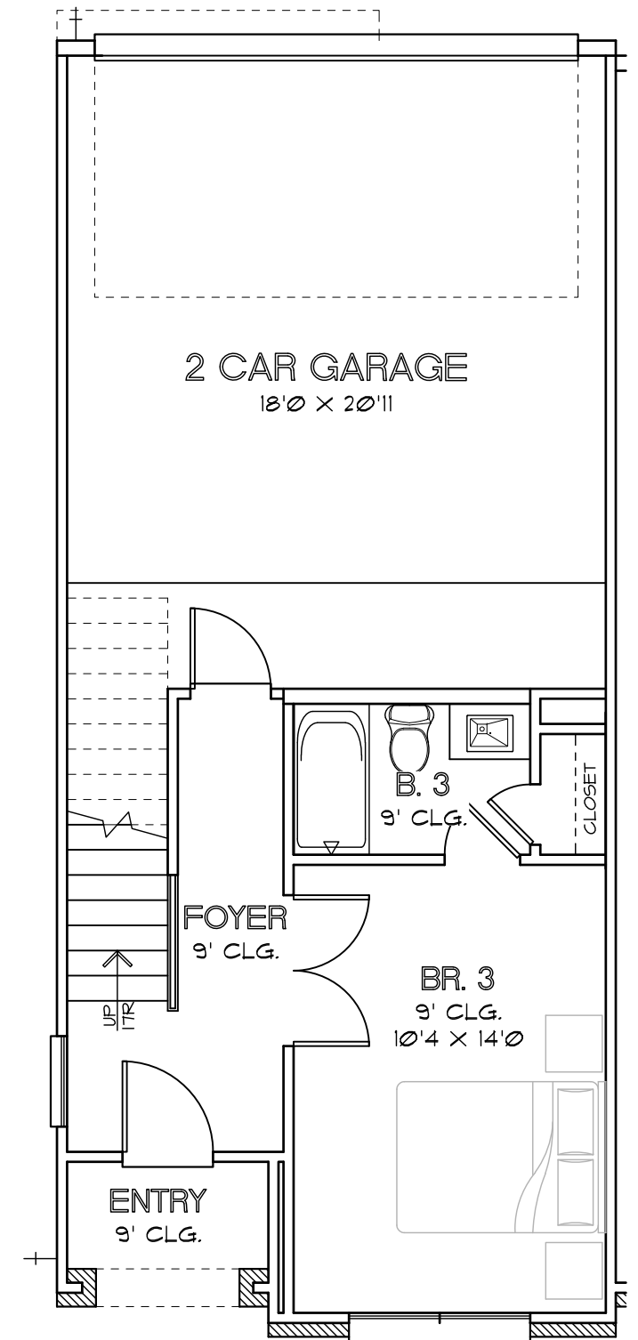
FIRST FLOOR PLAN PLAN 1870 L
