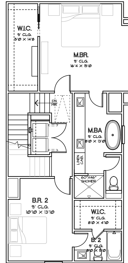
THIRD FLOOR PLAN PLAN 2101
