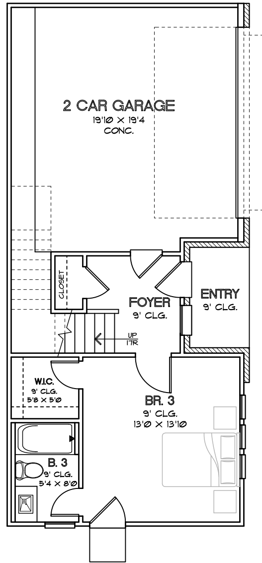
FIRST FLOOR PLAN PLAN 2101
