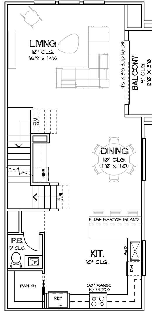
SECOND FLOOR PLAN PLAN 2101
