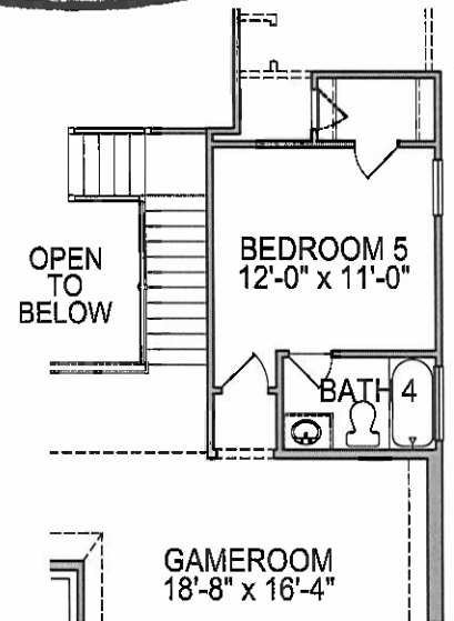
SECOND FLOOR PLAN OPT. #0094 BED 5/BATH 4 FROM ATTIC
