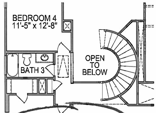
SECOND FLOOR PLAN OPT. #0113 CURVED STAIRS
