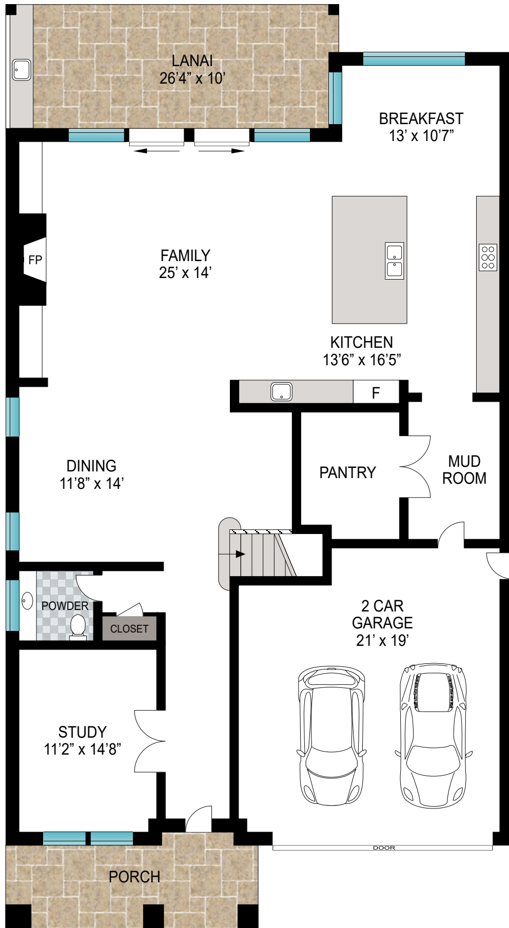
FIRST FLOOR
