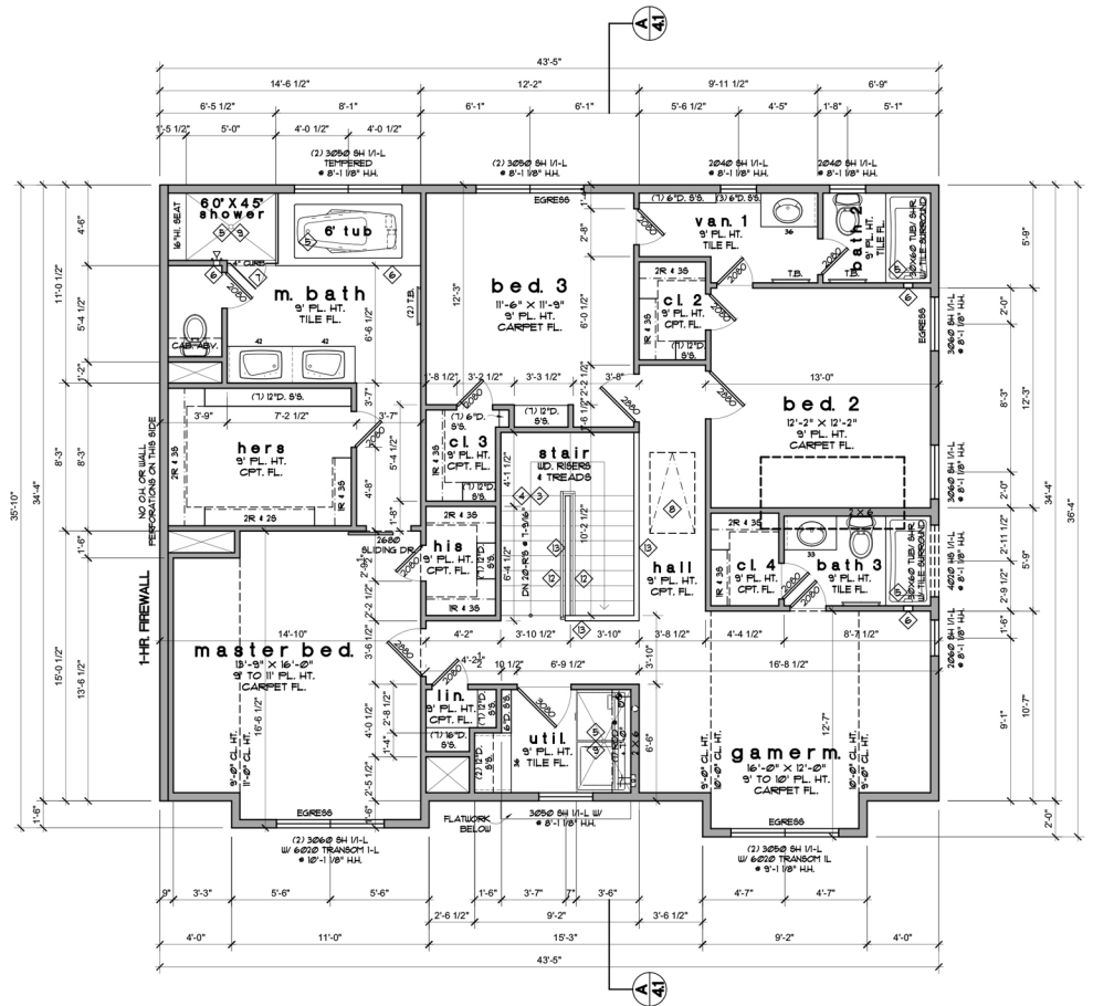
Second Floor
