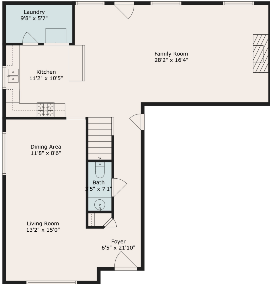
Floor 1
