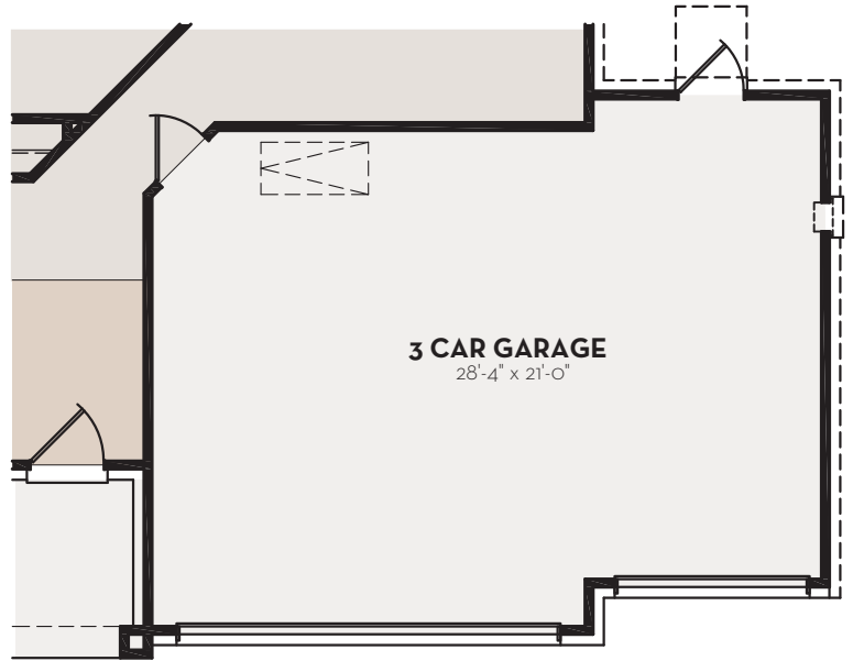
3 CAR GARAGE 28'-4" x 21'-0"
