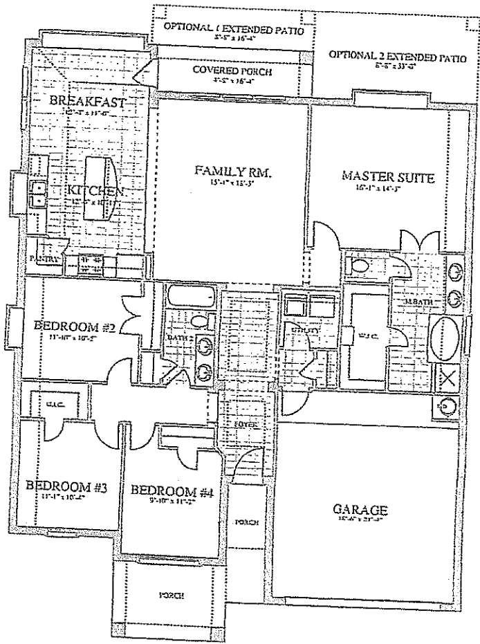
FLOOR PLAN 1853 S.F.
