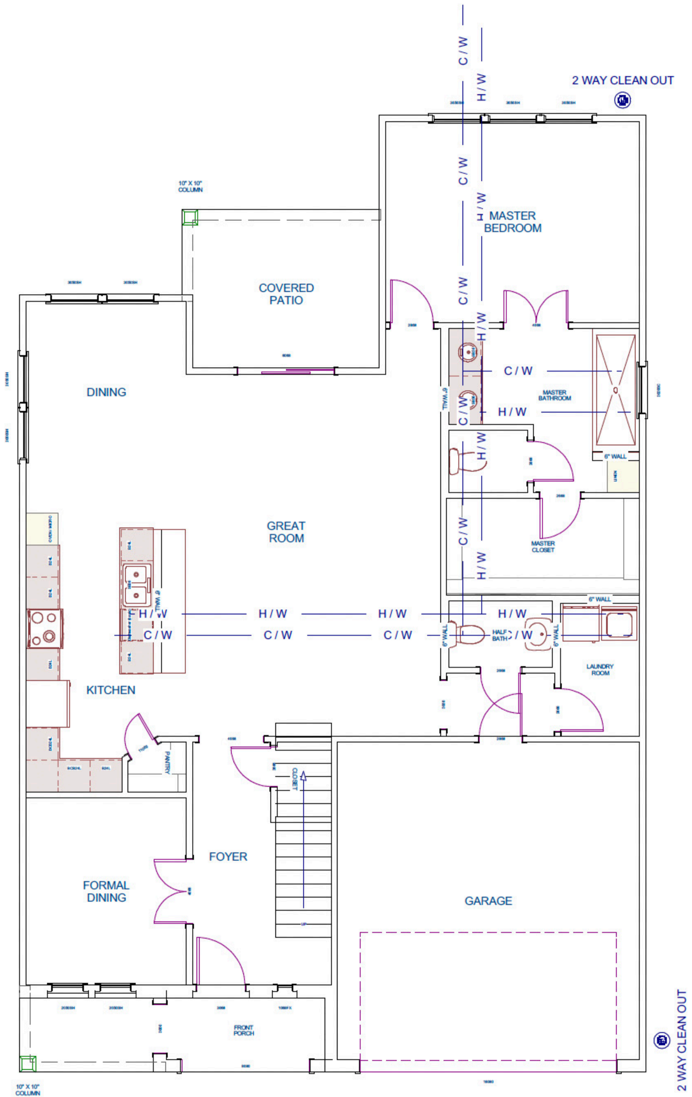
1st Floor
