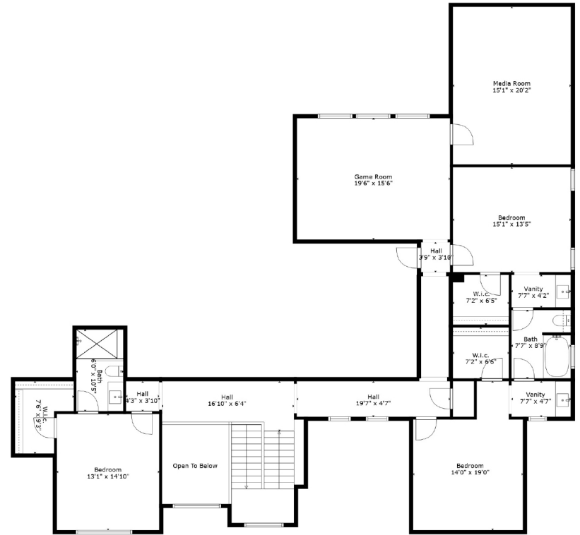
Floor 2
