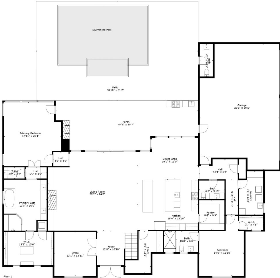
Floor 1
