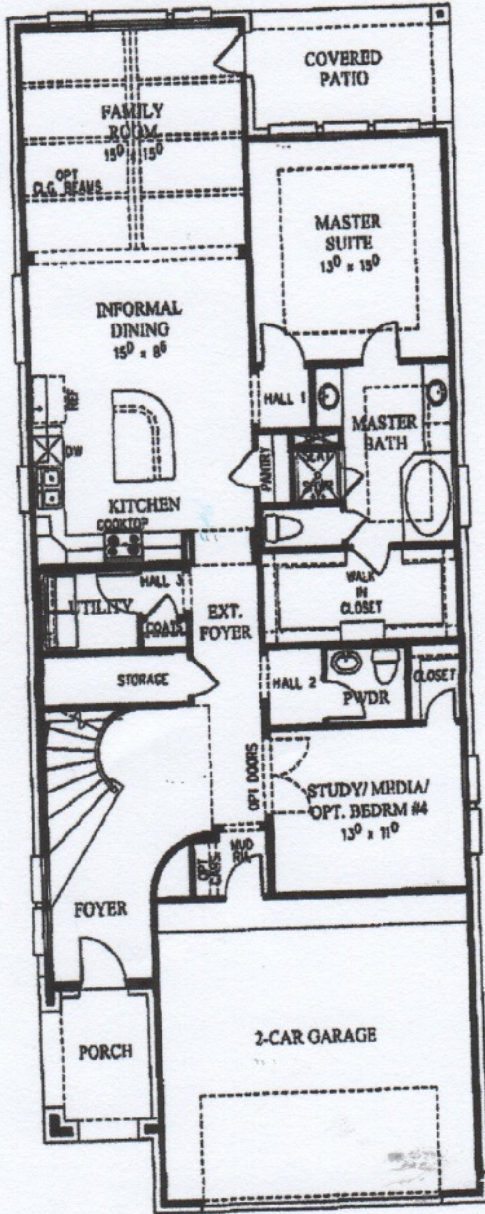
FIRST FLOOR
