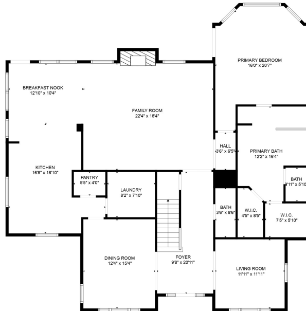
FLOOR 1
