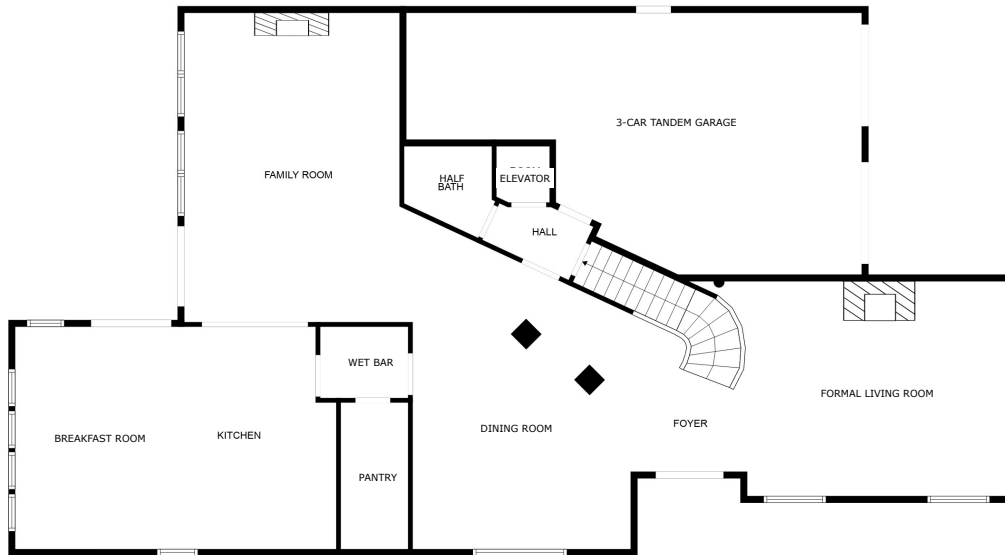
FLOOR 1
