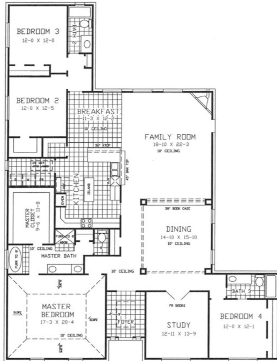
407 PLAN 3071 SQ. FT.
