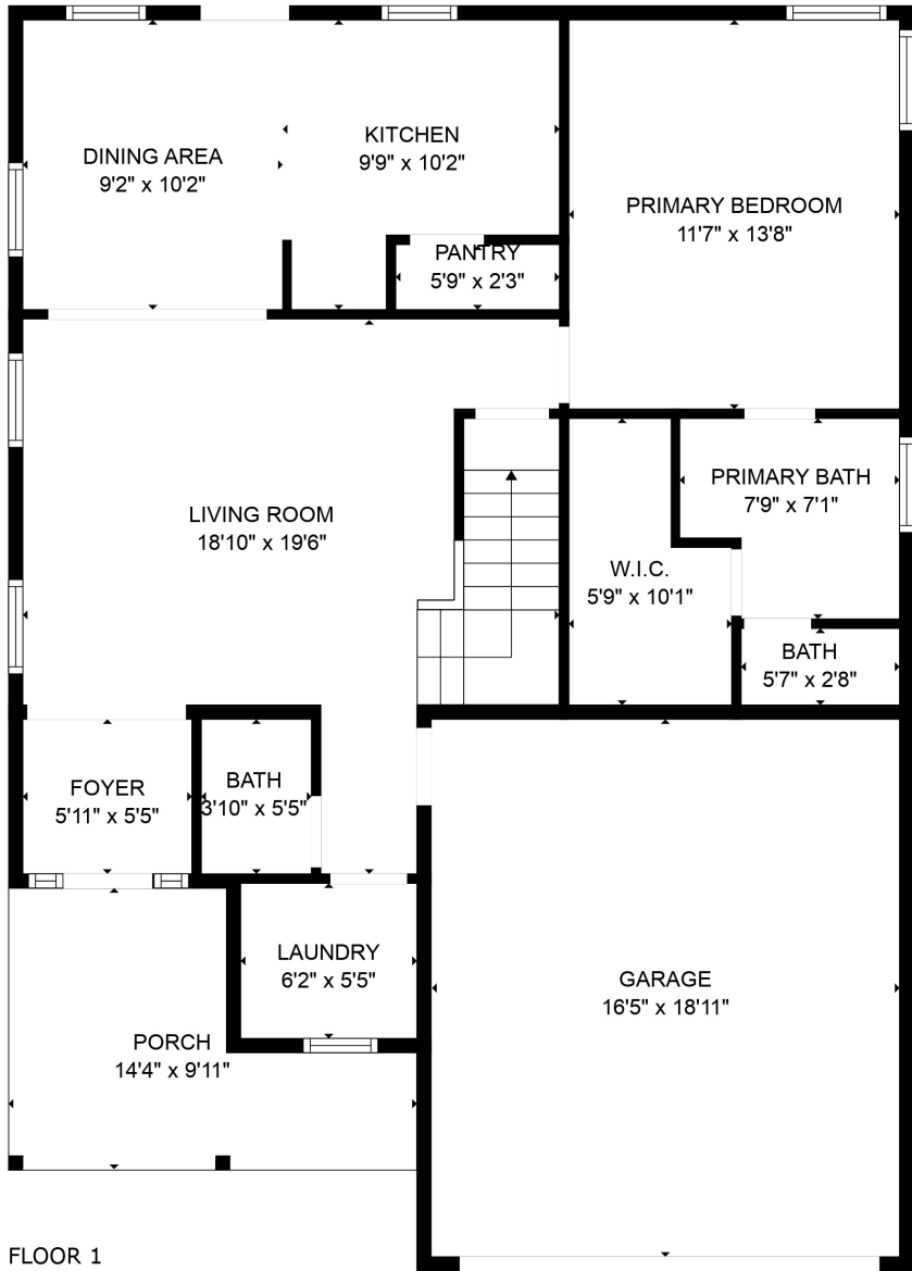
FLOOR 1
