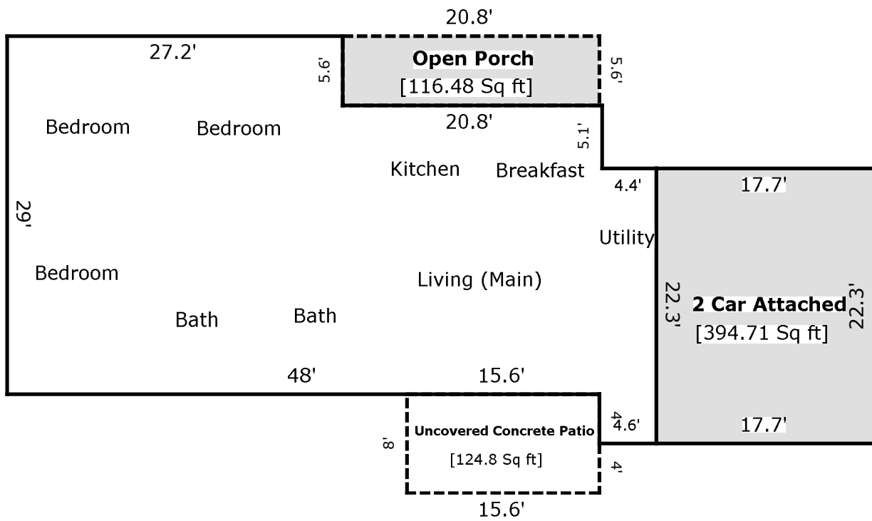
First Floor [1379.12 Sq ft]
